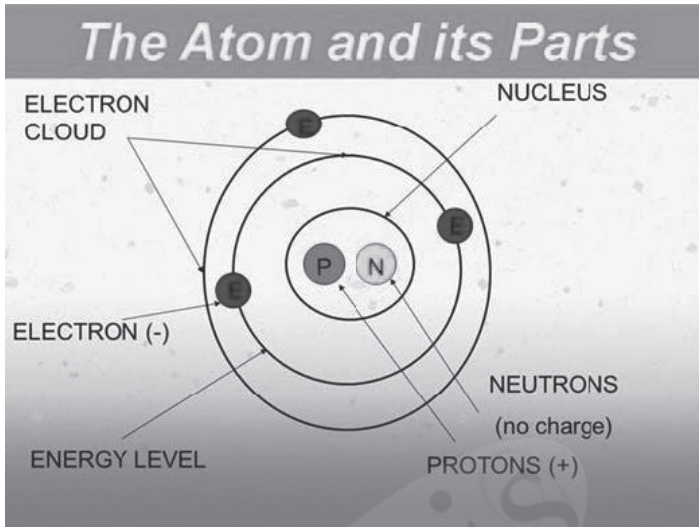
Figure 8. Every Atom has One or More Electrons that Orbits its Nucleus.
