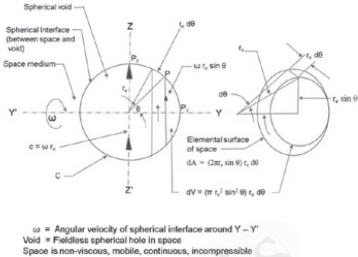
Figure 3. Velocity Field of the Electron Vacuum Space Vortex
